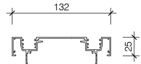
PAS340 132 DOUBLE GLAZING FRAME
