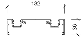
PAS335 132 DOUBLE GLAZING MULLION FRAME
