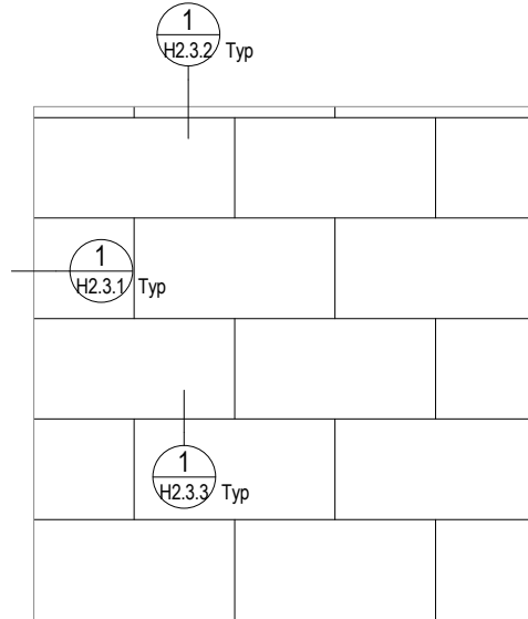
Potters Heradesign® Ceiling Direct Fix System (Stretcher Bond pattern)
