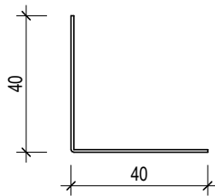
40x40 BULKHEAD ANGLE
