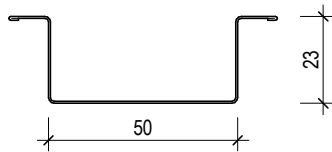
HERA CEILING/WALL BATTEN
