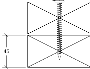
TIMBER DETAIL
