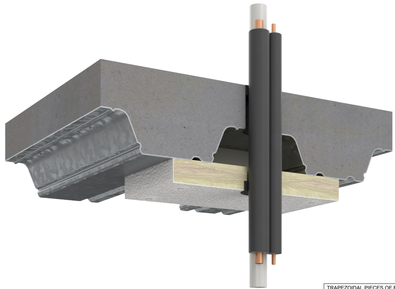
TRAPEZOIDAL PIECES OF BOSS BATT TO BOTH SIDES OF PENETRATION
