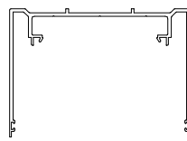
PAS425 132 DEFLECTION TRACK +/- 40MM
