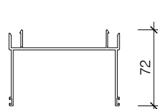
PAS426 132 DEFLECTION TRACK ADAPTOR +/- 40MM
