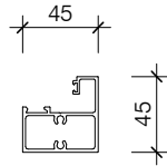
PAS004/GP45 SOHO 45MM GLAZING POST
