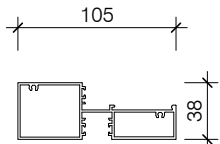
PAS021/A 105 GLAZING SILL/TRANSOM
