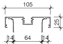
PAS014 105 PLASTERBOARD POCKET CAPPING FRAME
