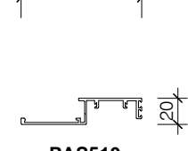
PAS510 SIDE ACOUSTIC SLIPPER CAPTURE PLATE
