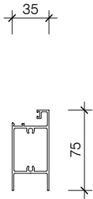
PAS503 75MM TOP & BOTTOM RAIL
