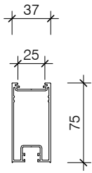
PAS500 75MM DOOR STILE
