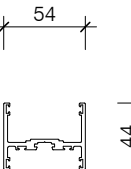
PAS520 SLIDING DOOR LOCATING FRAME
