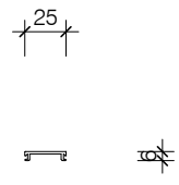
PAS502 FLAT SLIPPER PLATE
