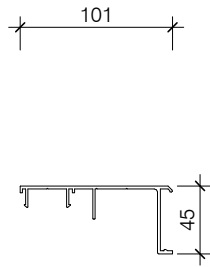
PAS530 STARTING FRAME
