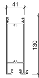
PAS532 GLAZING RAIL
