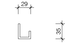
GUIDE TRACK
