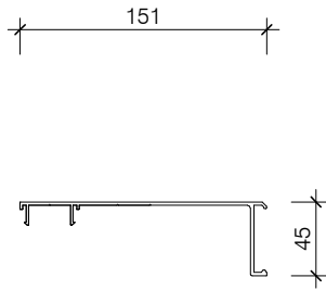
PAS530/D DOUBLE STARTING FRAME
