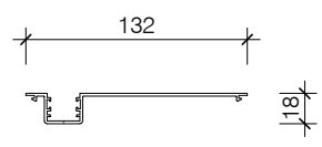
PAS338 132 OFFSET GLAZE SNAP IN POCKET
