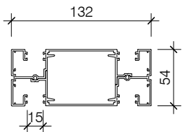
PAS343 TWO PIECE TWIN GLAZE MULLION
