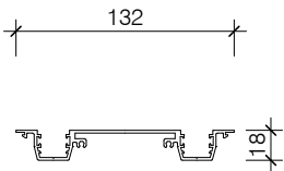
PAS339 132 TWIN GLAZE SNAP IN POCKET
