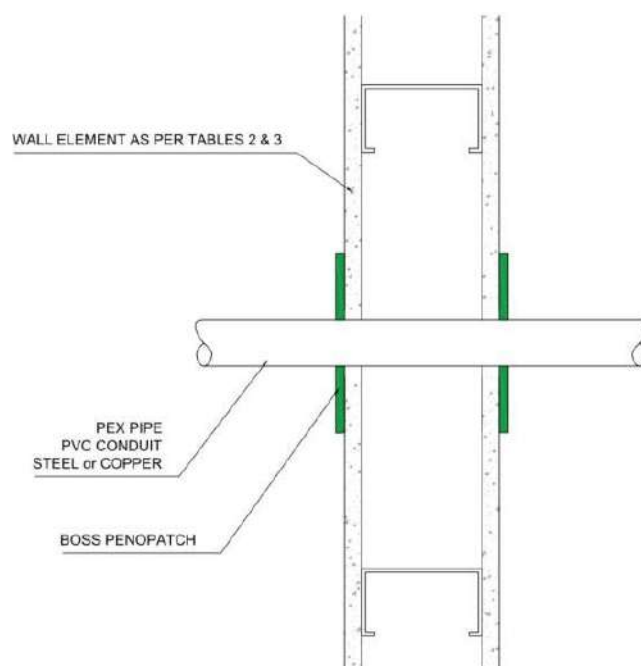
Figure 2 – PEX Pipe, PVC Conduit , Steel or Copper Penetrations
