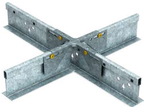
XD35 Seismic Separation Joint Clip
