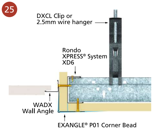
■ STANDARD OFFSET TRANSITION
