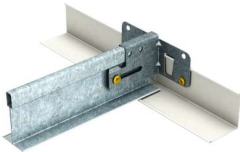
XD17 Seismic Clip, Grid to Wall Angle
