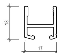
4.75MM FLATLINE 467355
