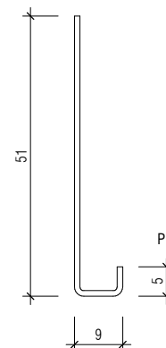
FIXING CLIP 350539
