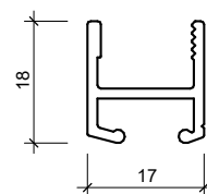
467375 12MM FLATLINE
