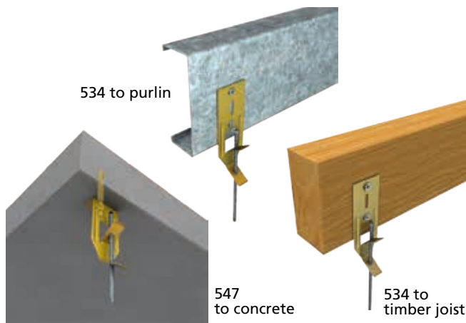
FIGURE 6: HANGER CLIPS
