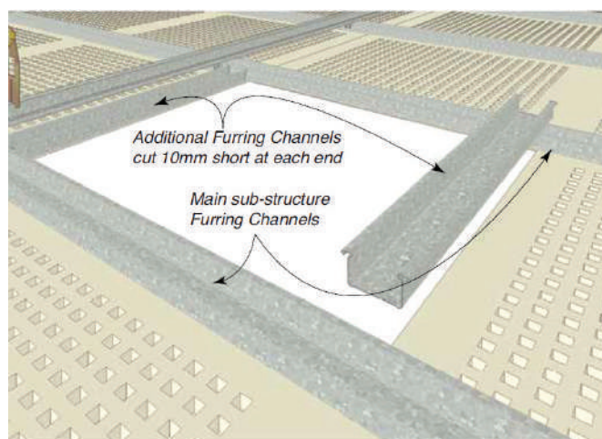
Figure 35: Back Blocking
