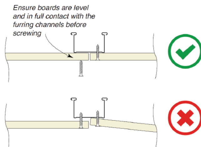
Figure 10: Board Support
