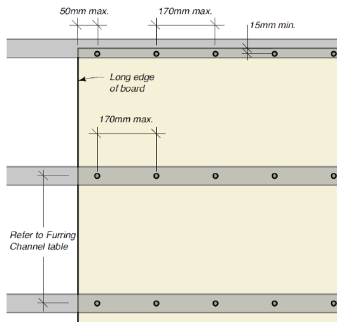
Figure 10: Board Support
