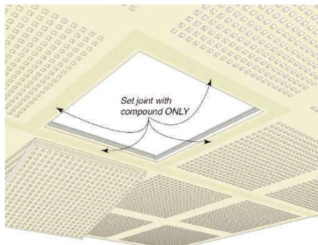
Figure 37: Frame Jointing
