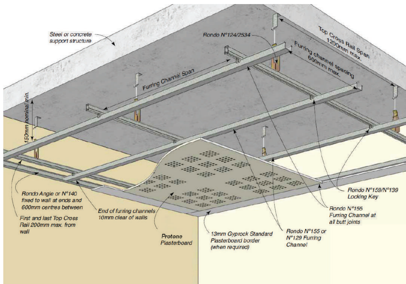
Figure 30 : Protone Concealed Grid Suspended Ceiling
