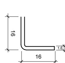
481120 FIXING ANGLE
