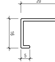
12MM EDGELINE 467372
