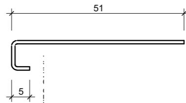
350539 FIXING CLIP
