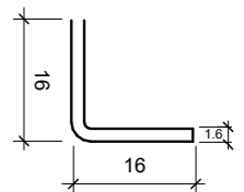
481120 FIXING ANGLE
