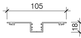
PAS016 POCKET DOORFRAME SNAP IN
