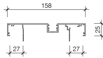
PAS314/DD GLAZING POCKET DOUBLE DOUBLE
