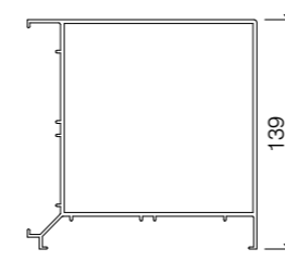
PAS324/JX 90° CORNER POST
