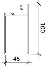
PAS003 BEADED POST
