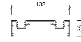
PAS335 TWIN GLAZE 36MM MULLION
