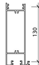
PAS532 500 SERIES GLAZING RAIL
