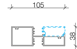
PAS021/A + PAS022 GLAZING SILL/TRANSOM
