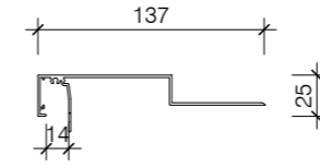
PAS313/B ADJ MULTI TRACK B
