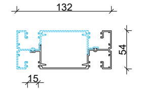
PAS343 TWO PIECE TWIN GLAZE MULLION
