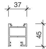
PAS500/45 SOHO 45MM DOOR STILE
