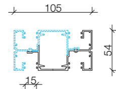
PAS043 TWO PCE MULLION TWIN GLAZED
