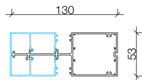
PAS321/B + PAS320 TRANSOM/MULLION/DOOR FRAME + GLAZING BEAD
