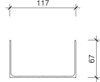
PAS327 132 DEFLECTION BASE U CHANNEL
