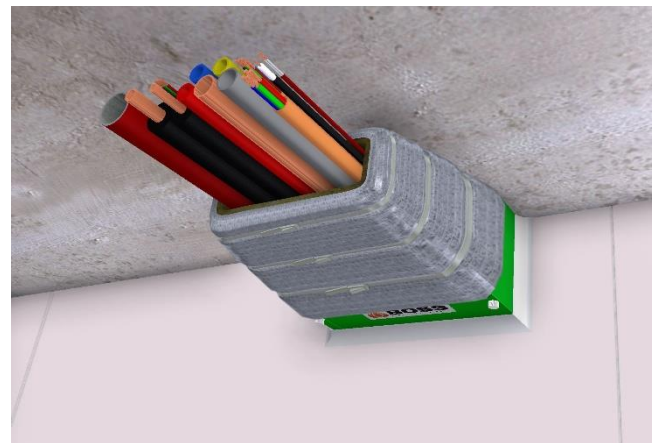
Above: BOSS FyreBox™
