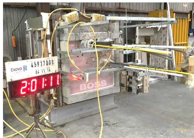
The BOSS FyreBox™ shown on the right during a fire test just after 120 minutes.
