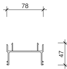
PAS026 105 DEFLECTION TRACK ADAPTOR
