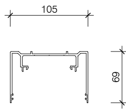
PAS025 105 DEFLECTION TRACK
