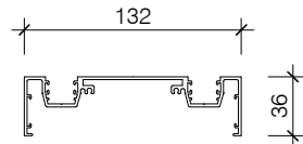
PAS335 132 TWIN GLAZING MULLION FRAME
