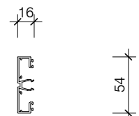
PAS342 TWIN GLAZING TRANSOM BEAD
