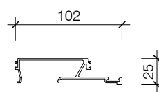
PAS336 132 TWIN GLAZING BEAD
