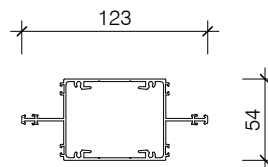
PAS341 TWIN GLAZING TRANSOM
