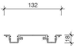
PAS339 132 TWIN GLAZE SNAP IN POCKET
