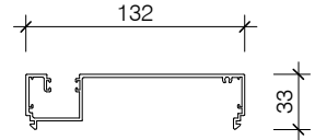
PAS332/D 132 DEEP POCKET GLAZING FRAME
