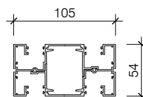
PAS043 TWO PCE MULLION TWIN GLAZED
