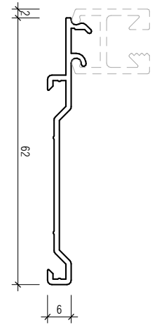
PEN TRAY WITH FLATLINE 467369
