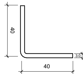
351596 FIXING ANGLE
