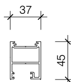
PAS500/45 SOHO 45MM DOOR STILE
