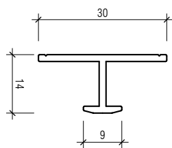
9MM H JOINTER 467380
