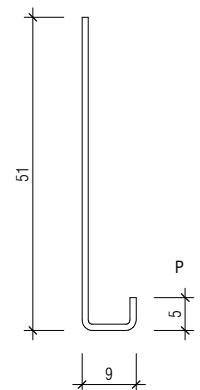
FIXING CLIP 350539
