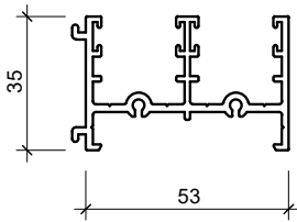
467364 CABINET SLIDER DOUBLE TRACK
