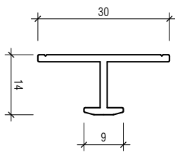
9MM H JOINTER 467380
