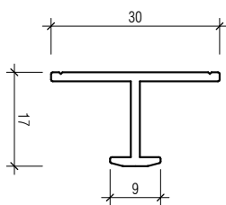
12MM H JOINTER 467382
