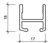
467375 12MM FLATLINE
