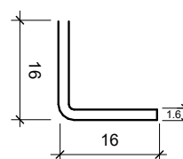
481120 FIXING ANGLE
