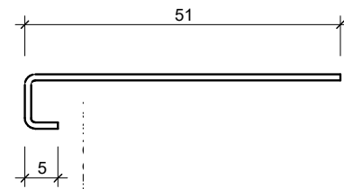
350539 FIXING CLIP
