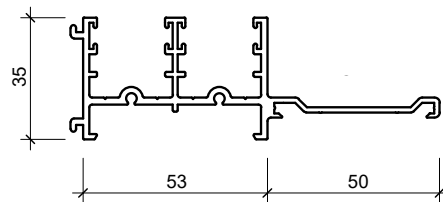
467366 CABINET SLIDER DOUBLE TRACK WITH PEN TRAY
