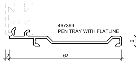
467369 PEN TRAY WITH FLATLINE
