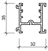
467361 CABINET SLIDER SINGLE TRACK
