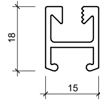
467355 4.75MM FLAT LINE
