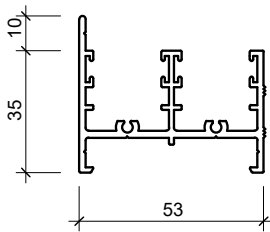
467357 COUNTERBALANCE FRAME
