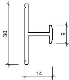
467380 9MM H JOINTER
