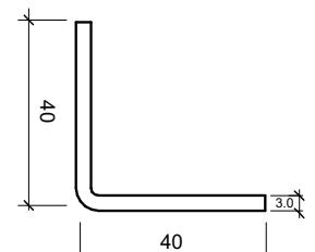
351596 FIXING ANGLE
