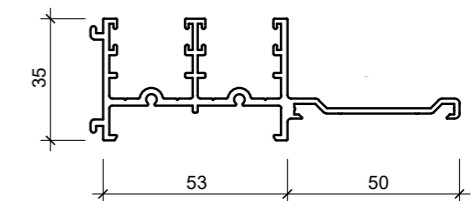
467366 CABINET SLIDER DOUBLE TRACK WITH PEN TRAY
