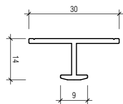
9MM H JOINDER 467380
