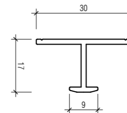
12MM H JOINDER 467382
