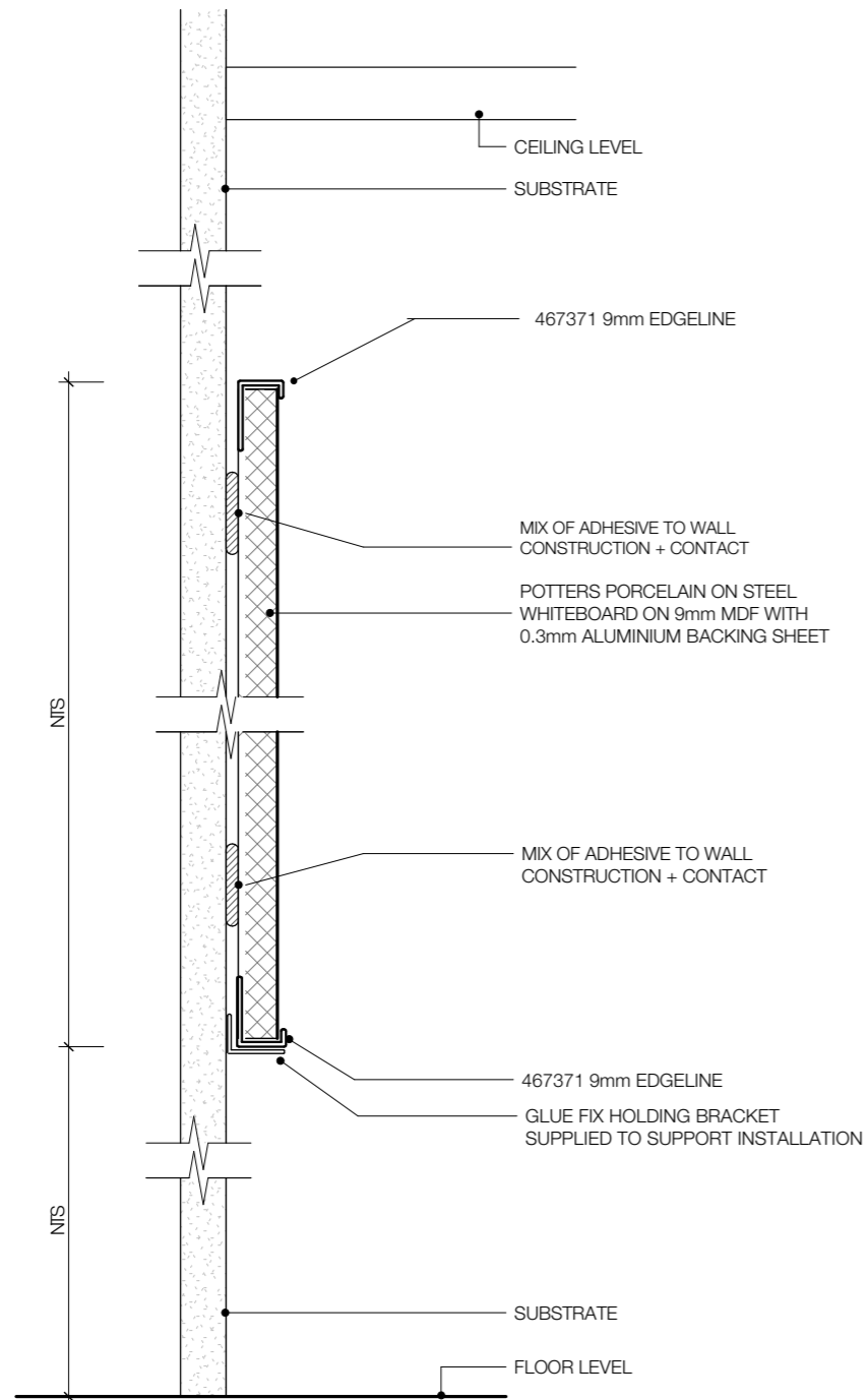
WHITEBOARD GLUE FIXED INSTALL - 9MM SUBSTRATE
