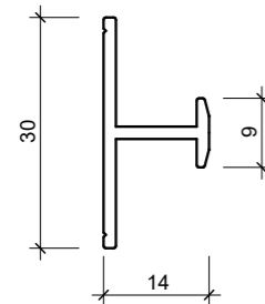
467380 9MM H JOINTER
