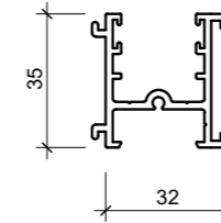
467361 CABINET SLIDER SINGLE TRACK
