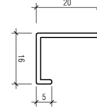
12MM EDGELINE 467372
