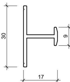
467382 12MM H JOINTER
