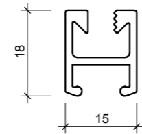
467355 4.75MM FLAT LINE
