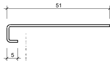
350539 FIXING CLIP
