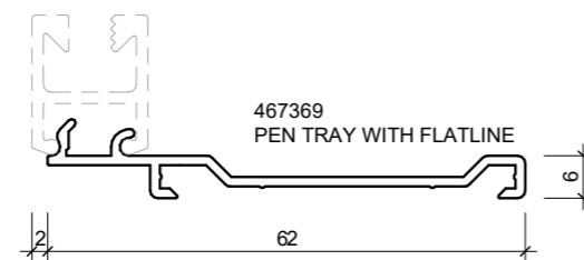
467369 PEN TRAY WHIT FLATLINE
