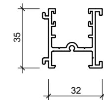
467361 CABINET SLIDER SINGLE TRACK
