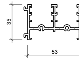
467364 CABINET SLIDER DOUBLE TRACK
