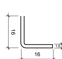
481120 FIXING ANGLE
