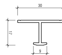
12MM H JOINTER 467382
