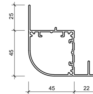
467384 LOCKABLE NOTICEBOARD FRAME
