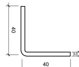
351596 FIXING ANGLE
