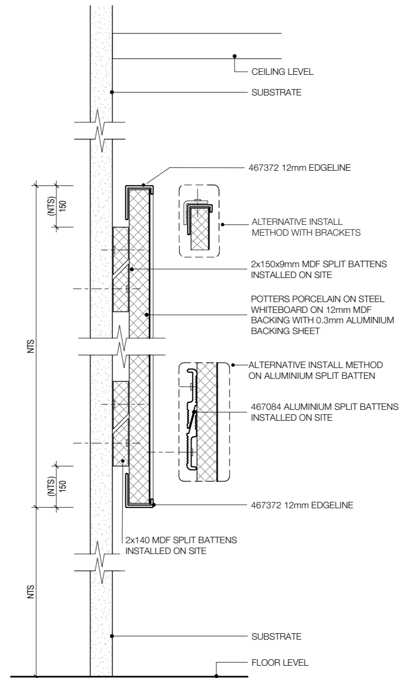
WHITEBOARD SPLIT BATTEN OR BRACKET INSTALL - 12MM SUBSTRATE
