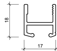
467375 12MM FLAT LINE
