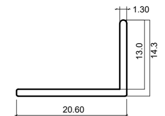
351595 12MM SLIMLINE BRACKET
